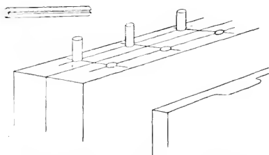
FIG. 253. DOWELED JOINT.
